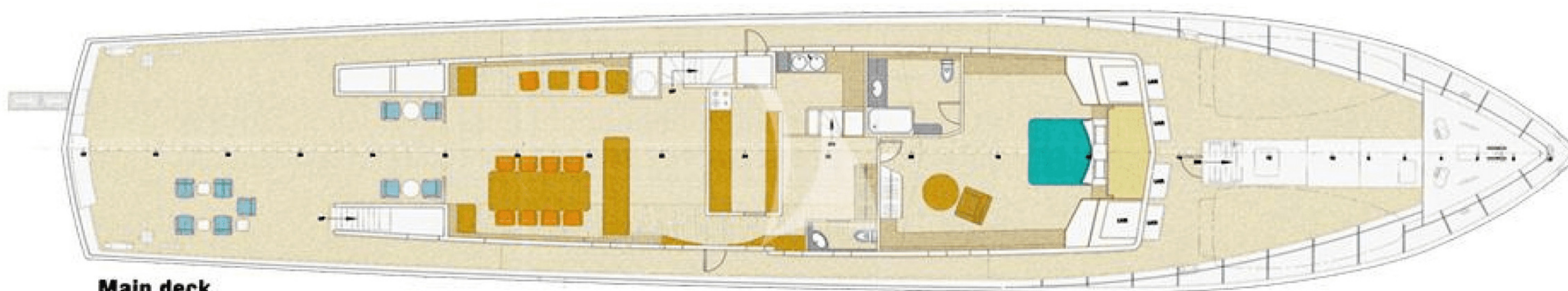
Main deck
